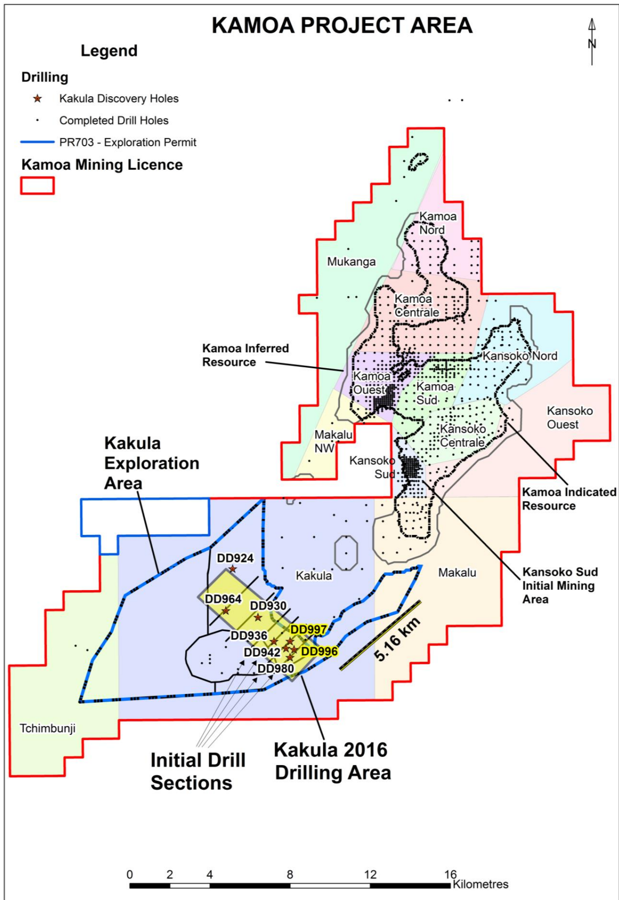
Figure 1: Kamoa plan map showing Kakula exploration area, discovery drill holes and 2016 drilling area.
