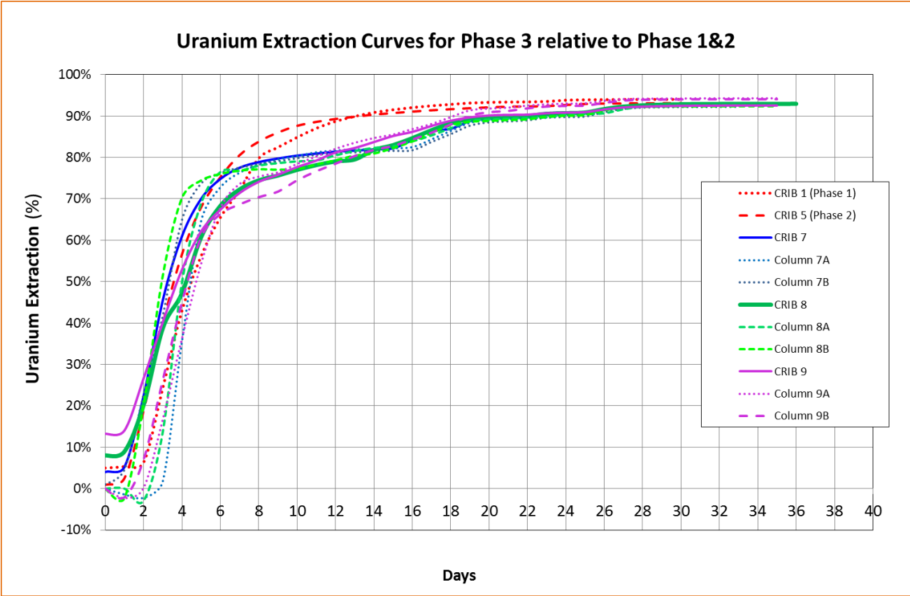
Figure 1 - Uranium extraction curves for Phase 3
