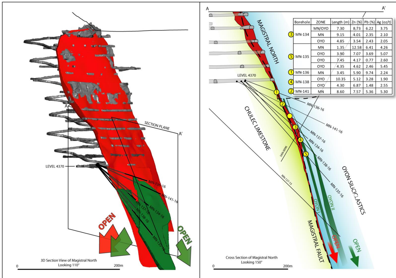
Figure 2: 3D view, looking SE and cross section illustrating geometry of the Oyon mineralization and location of recent drill hole intercepts at Magistral North and Oyon mantos.
