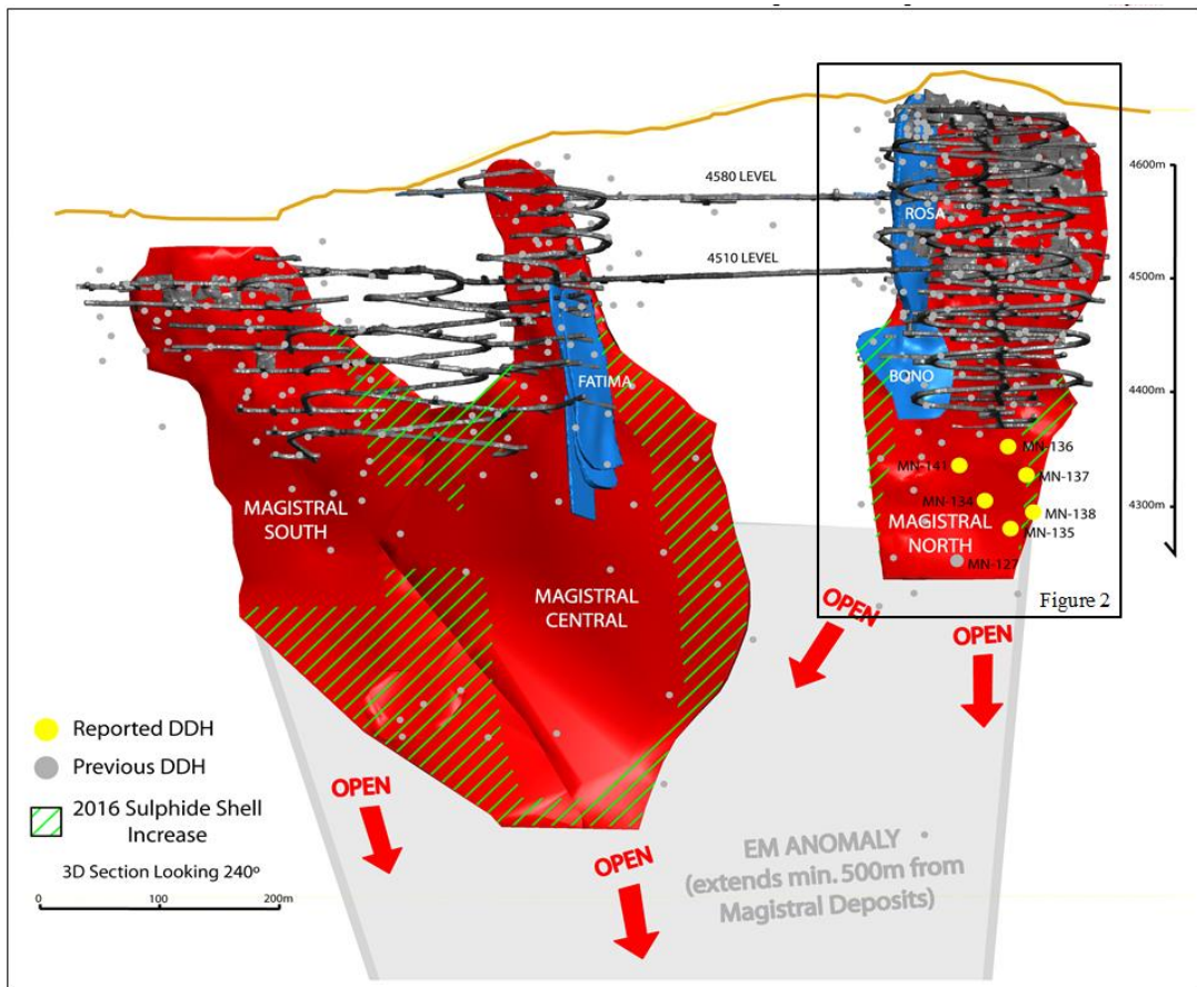
Figure 1: Long section looking west showing Magistral Deposits with reported drill hole intercepts
