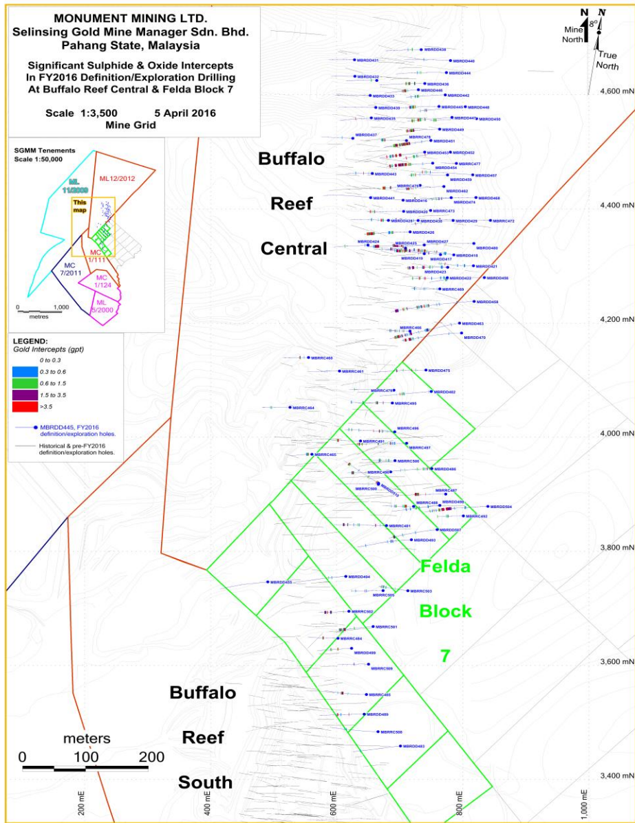
Figure 1–Drill hole Location Plan for composited assays greater than 1.0g/t
