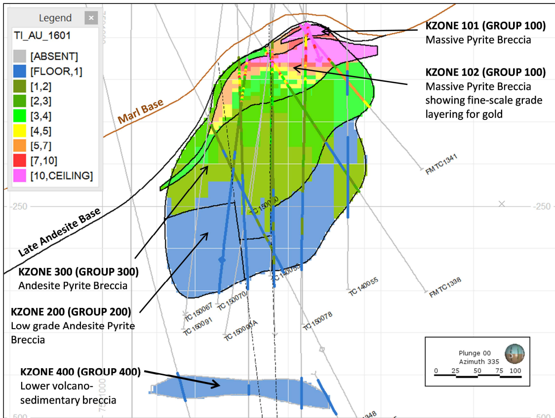
Cukaru Peki Block Model Gold (g/t) Grade Distribution view north to north-west
