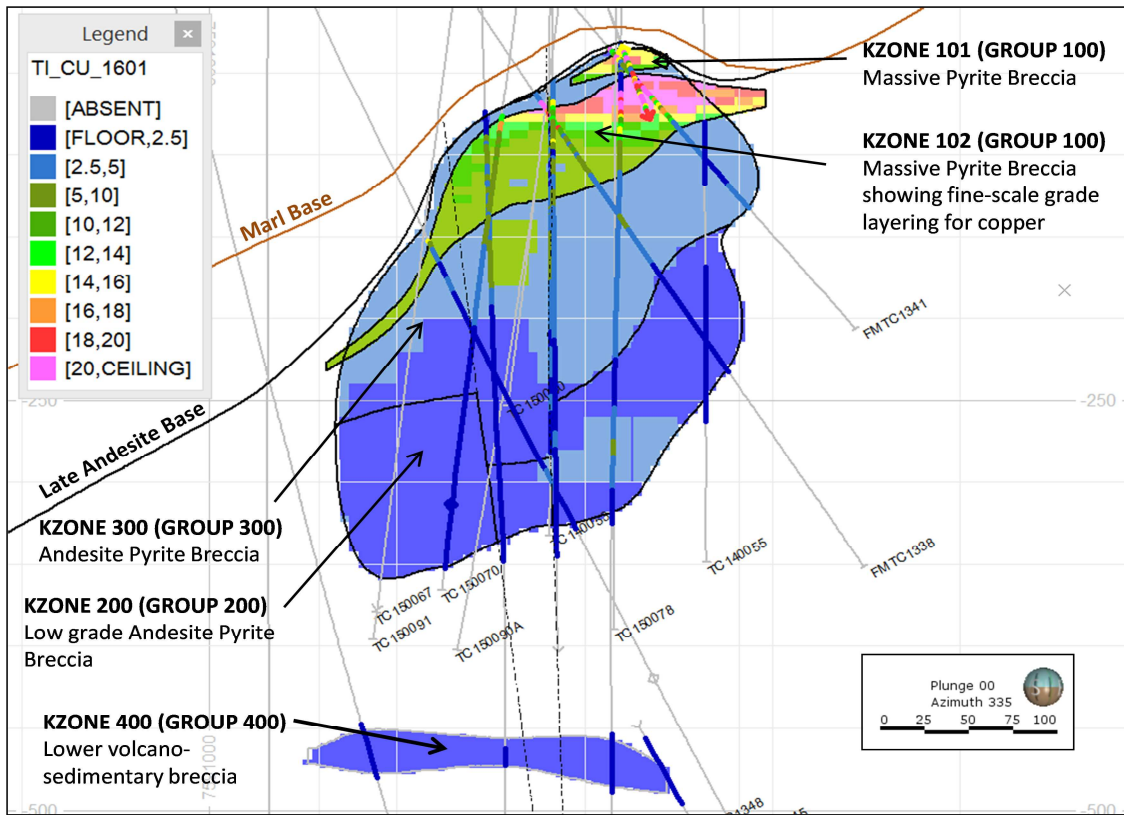
Cukaru Peki Block Model Copper (%) Grade Distribution looking north to northwest
