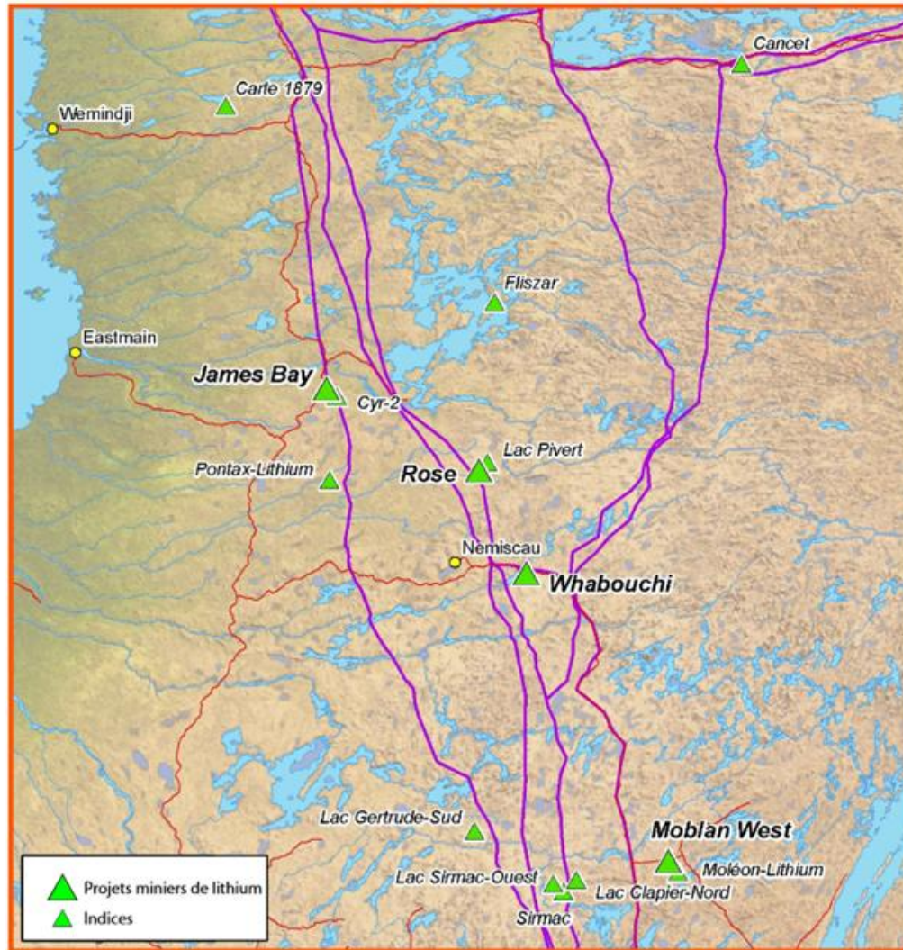
Figure 1. Location of known lithium deposits and occurrences in the James Bay area of Quebec (according to Quebec Ministry of Natural Resources and Fauna, 2011).
