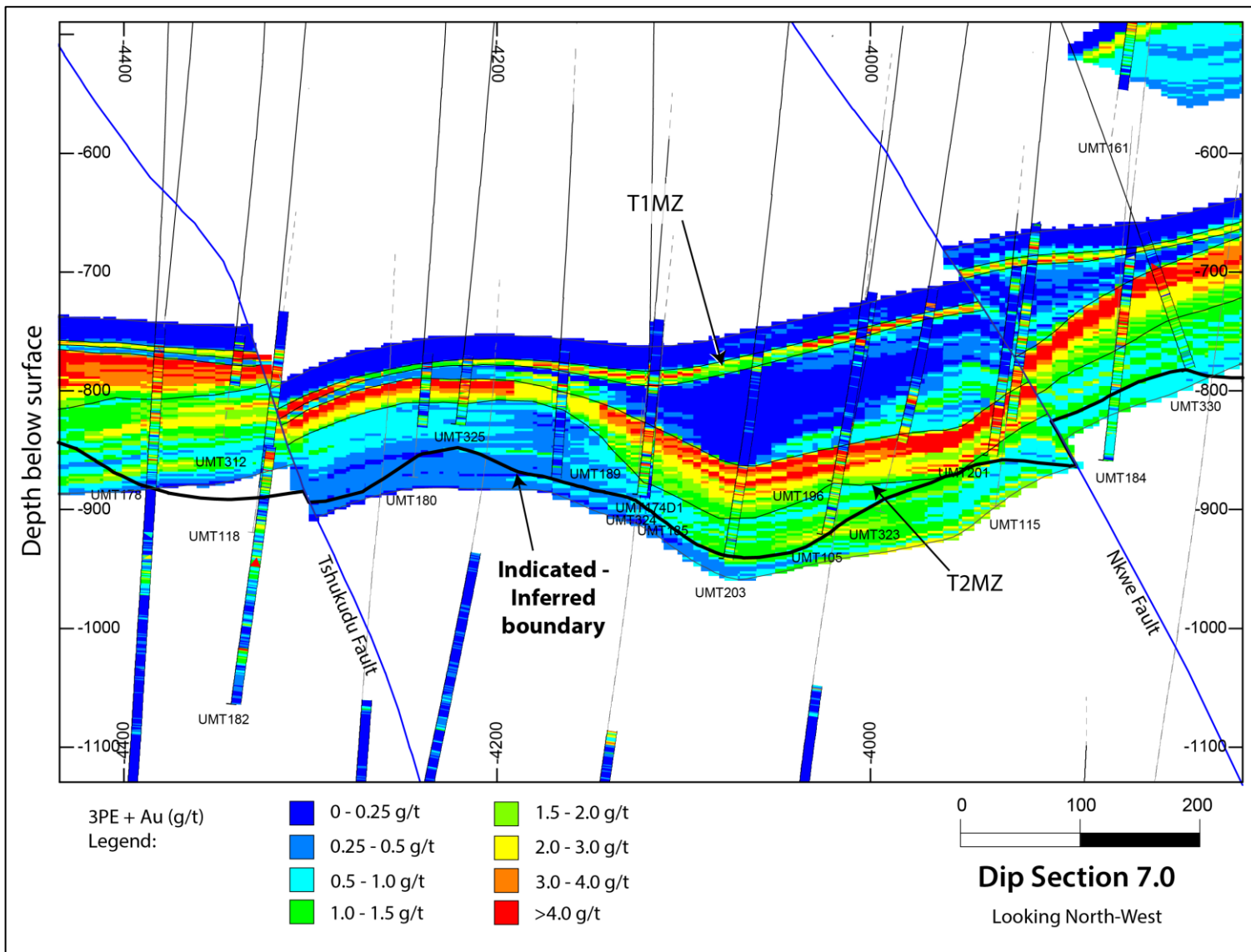
Figure 4: Flatreef cross section showing T1 and T2 mineralized zones (T1MZ and T2MZ), and the significant top loading of the T2 mineralized zone.
