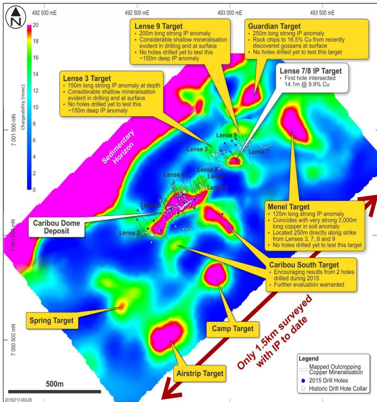
Figure 1. Plan view of inverted IP data acquired at the Caribou Dome Project during 2015. There is a strong correlation between IP anomalism and known mineralisation. The undrilled strong Menel, Guardian, Lense 9 and Lense 3 IP Targets are all located immediately along strike from the drill-tested mineralisation.
