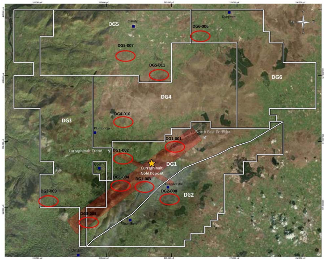
Figure 2: Dalradian licence areas with priority gold targets indicated by red ovals.
