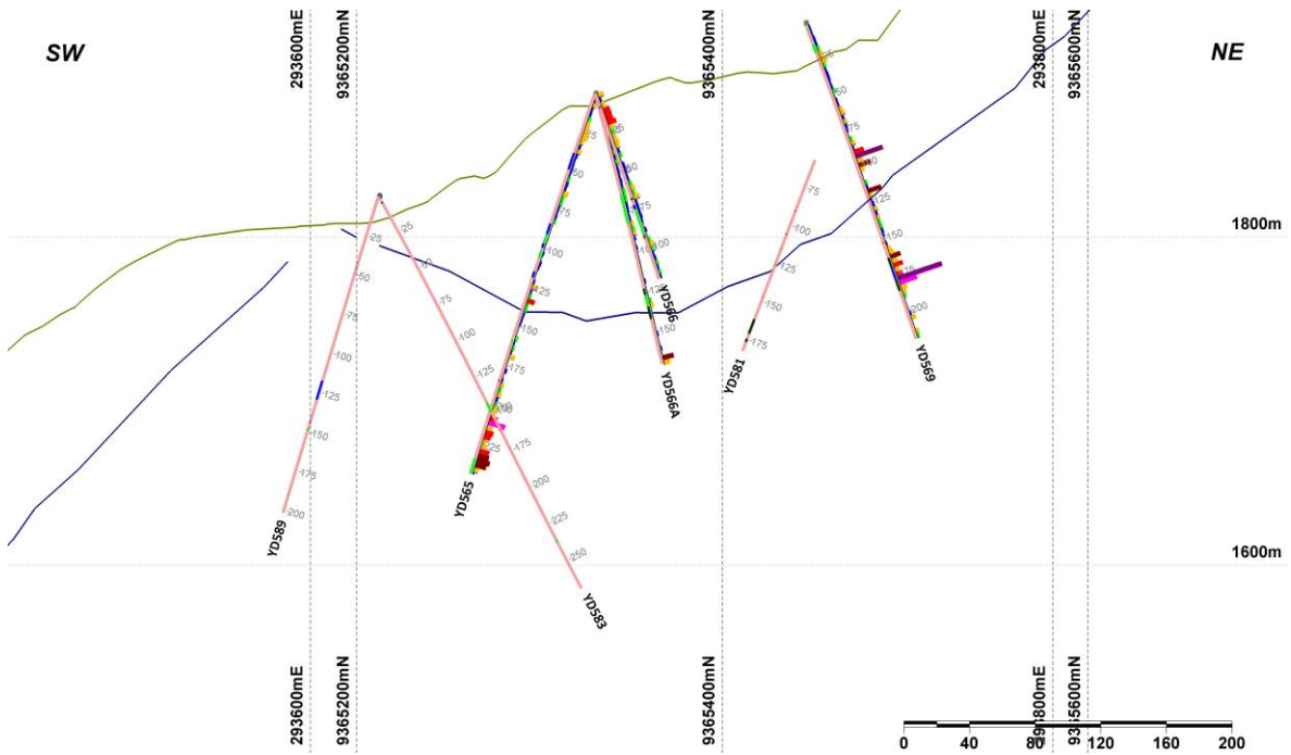
Figure 4. Section C-C'. This section is oriented southwest to northeast and the look direction is to the northwest. The brown line is the topography and the blue line is the bottom of the modeled open pit for the 2015 resource.
