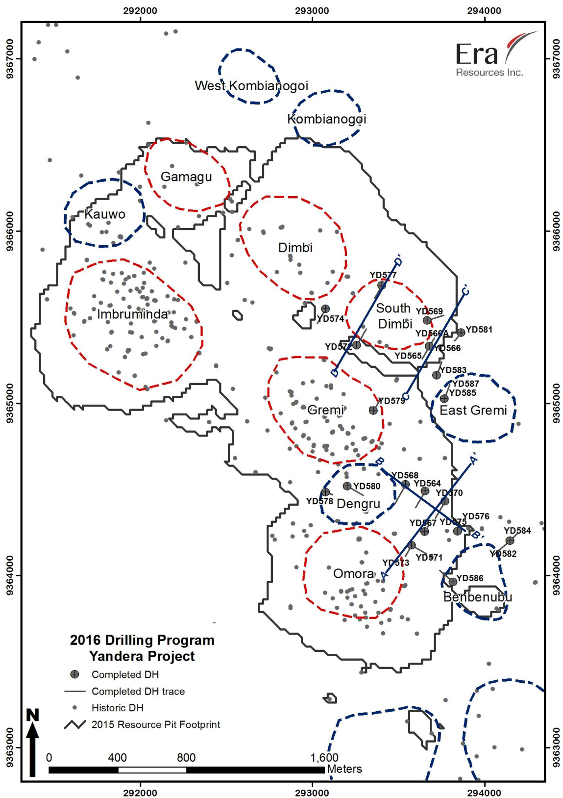
Figure 1. Yandera area prospects and deposits. The blue lines show the centerline of the sections below.
