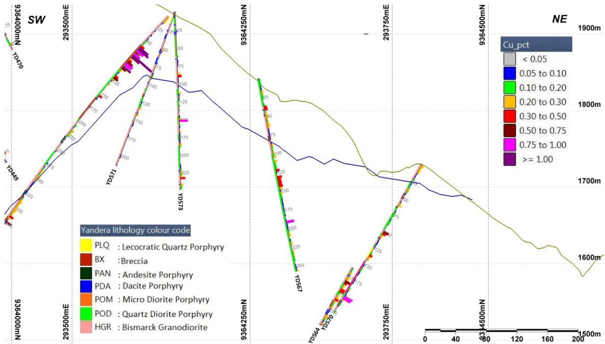
Figure 2. Section A-A'. This section is oriented southwest to northeast with the look direction to the northwest. The section width is 125 metres. The brown line is the topography and the blue line is the bottom of the modeled open pit for the 2015 resource. The right side of each drill trace shows copper values and the left side of each trace shows lithology. The legend in Section A-A' applies to all other sections.
