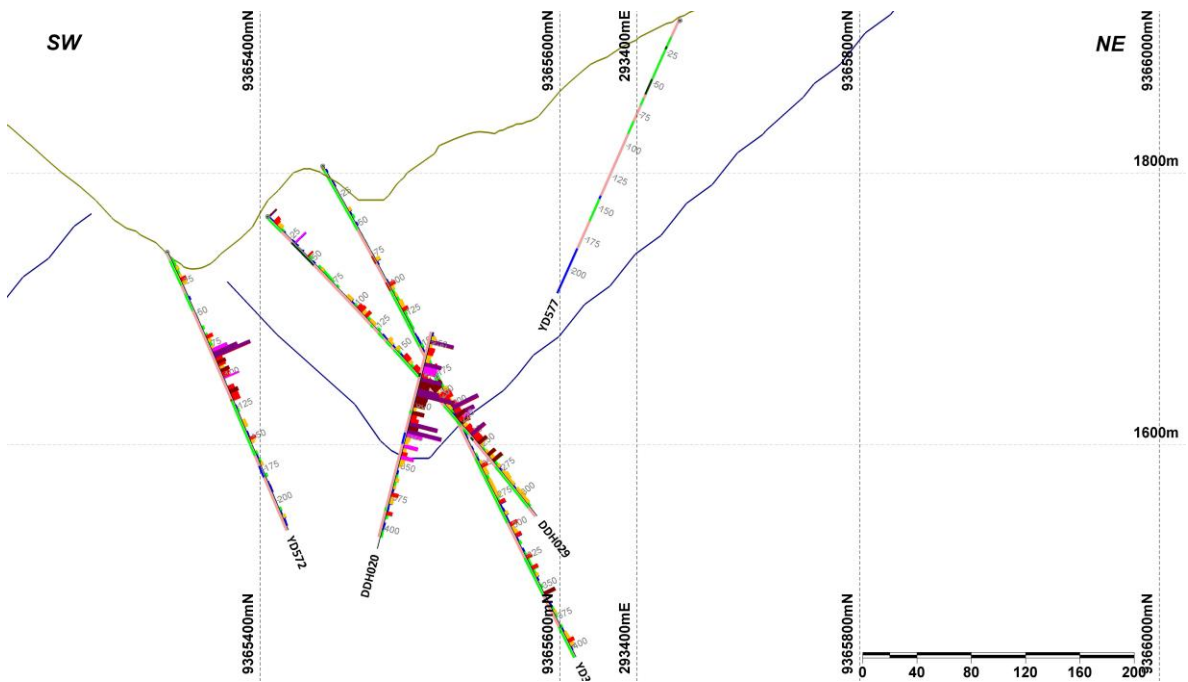
Figure 5. Section D-D'. This section is oriented southwest to northeast and the look direction is to the northwest. The brown line is the topography and the blue line is the bottom of the modeled open pit for the 2015 resource.
