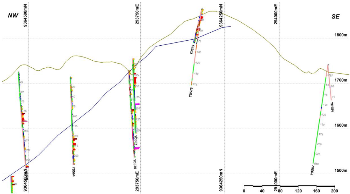
Figure 3. Section B-B'. This section is oriented northwest to southeast with the look direction to the northeast. The section width is 125 metres. The brown line is the topography and the blue line is the bottom of the modeled open pit for the 2015 resource.
