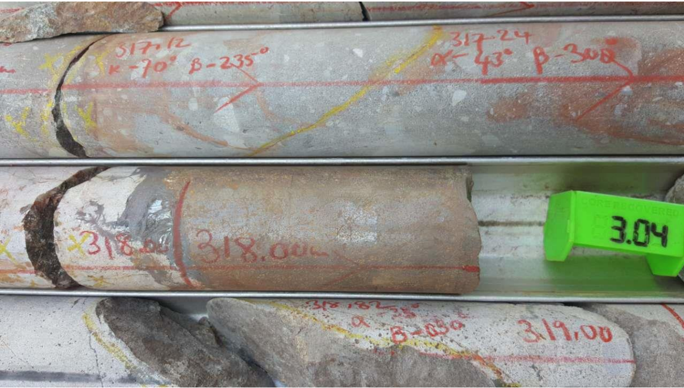
Figure 3. Intercept from DD1054, an in-fill hole near the centre of the Kakula Discovery, with massive chalcocite at a depth of 318 metres (chalcocite is approximately 80% copper by weight).
