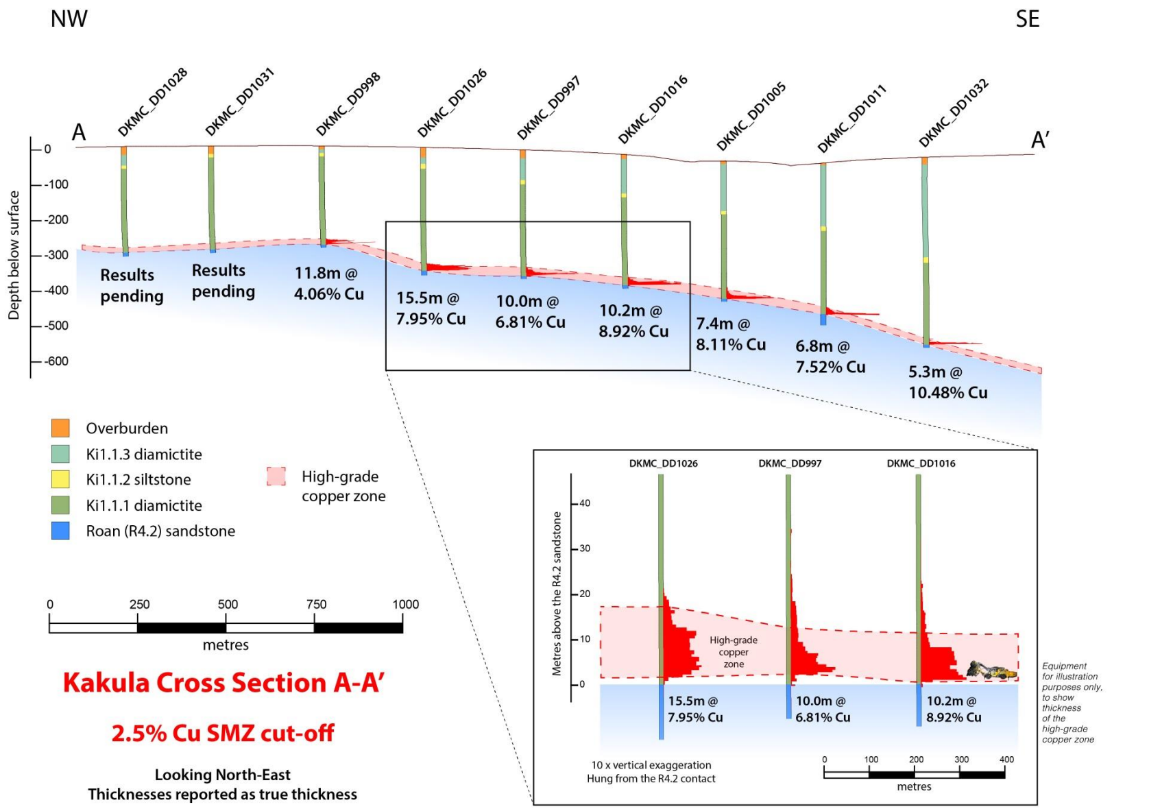
Figure 9. New cross-section A-A' of Kakula Discovery area, showing true thicknesses of drill intercepts at a 2.5% copper cut-off.
