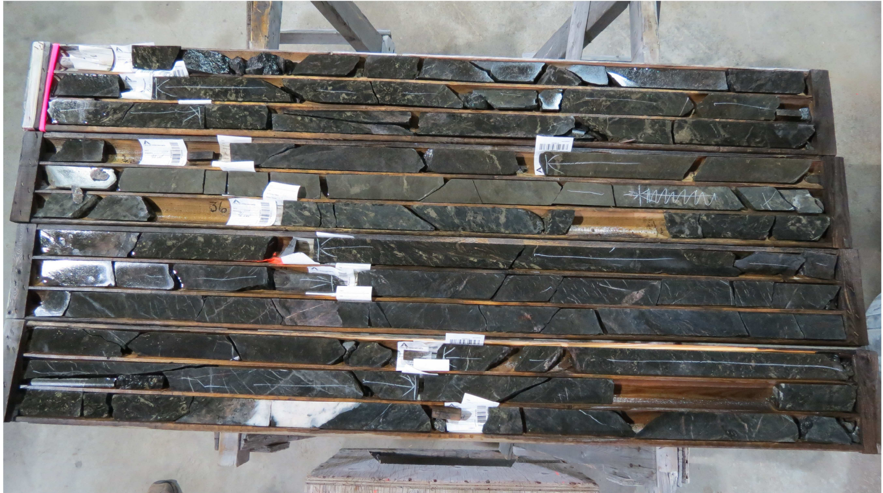
Figure 2. Chlorite bearing “feeder pipes” in DDH DO-92-24 yielding 18 meters of semi-massive pyrite stringers. NQ core with end of hole towards the lower right corner. Core box length is 1.5 meters.
