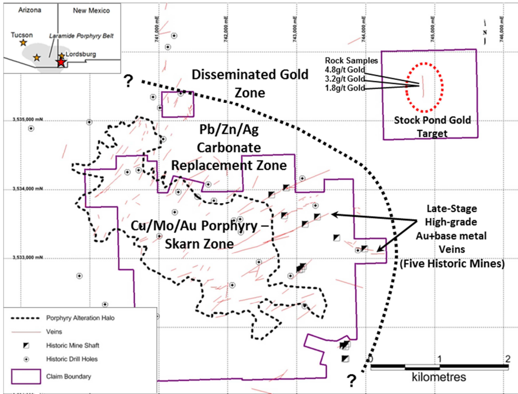
Figure 1: Metal zoning at the Oro project
