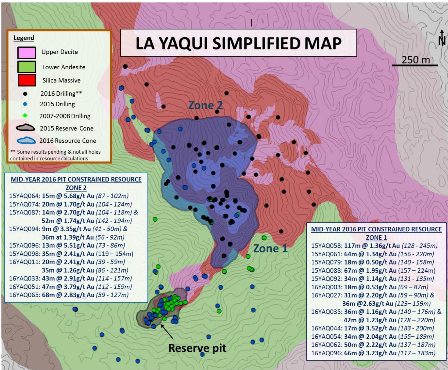
Figure 1: Greater Yaqui Project Area – Simplified Geology Map with Intercepts
