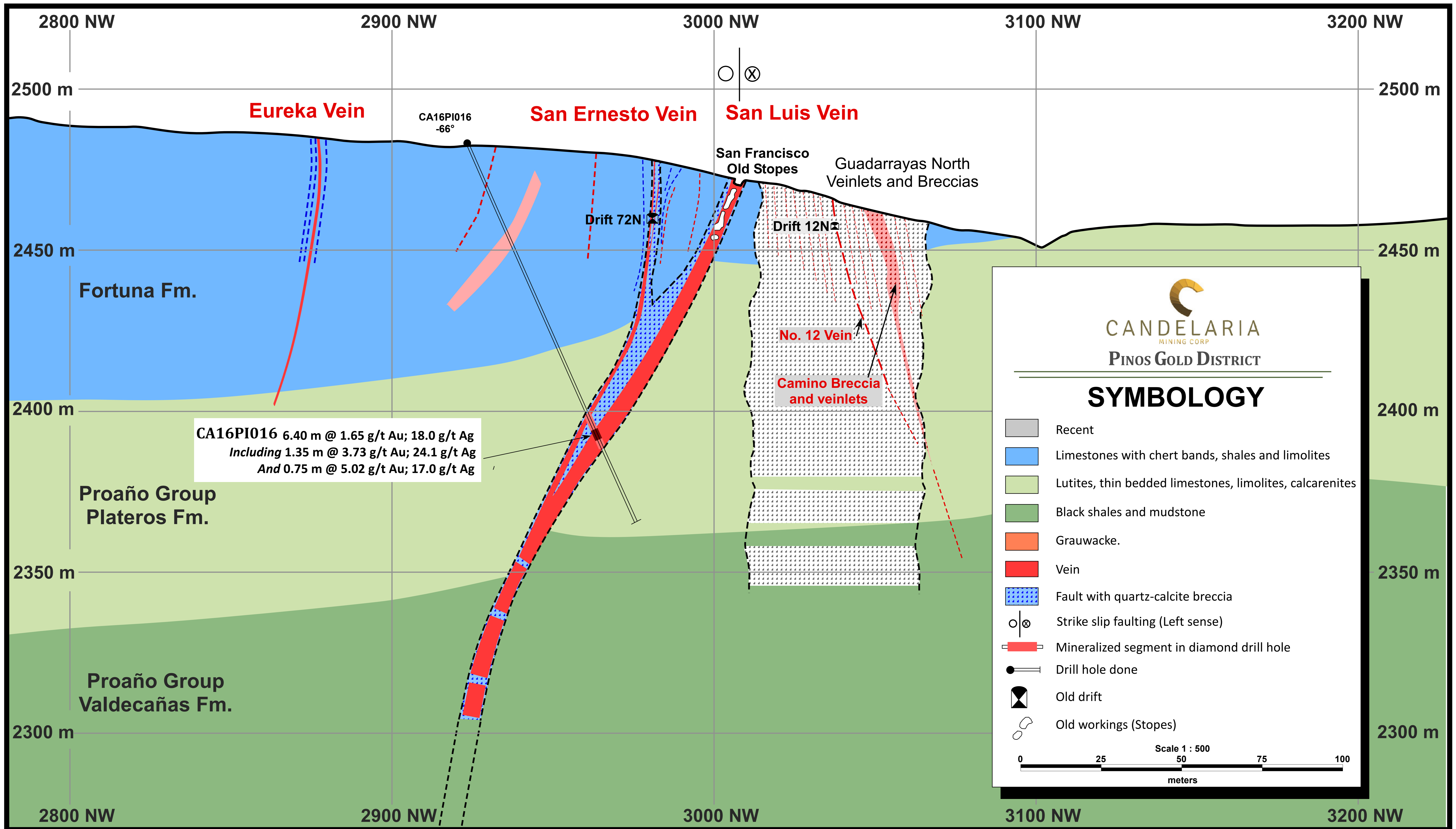
PINOS DISTRICT, TRANSVERSAL SECTION 9700 NE (LOOKING NW) SAN FRANCISCO CINCO ESTRELLAS VEINS SYSTEM
