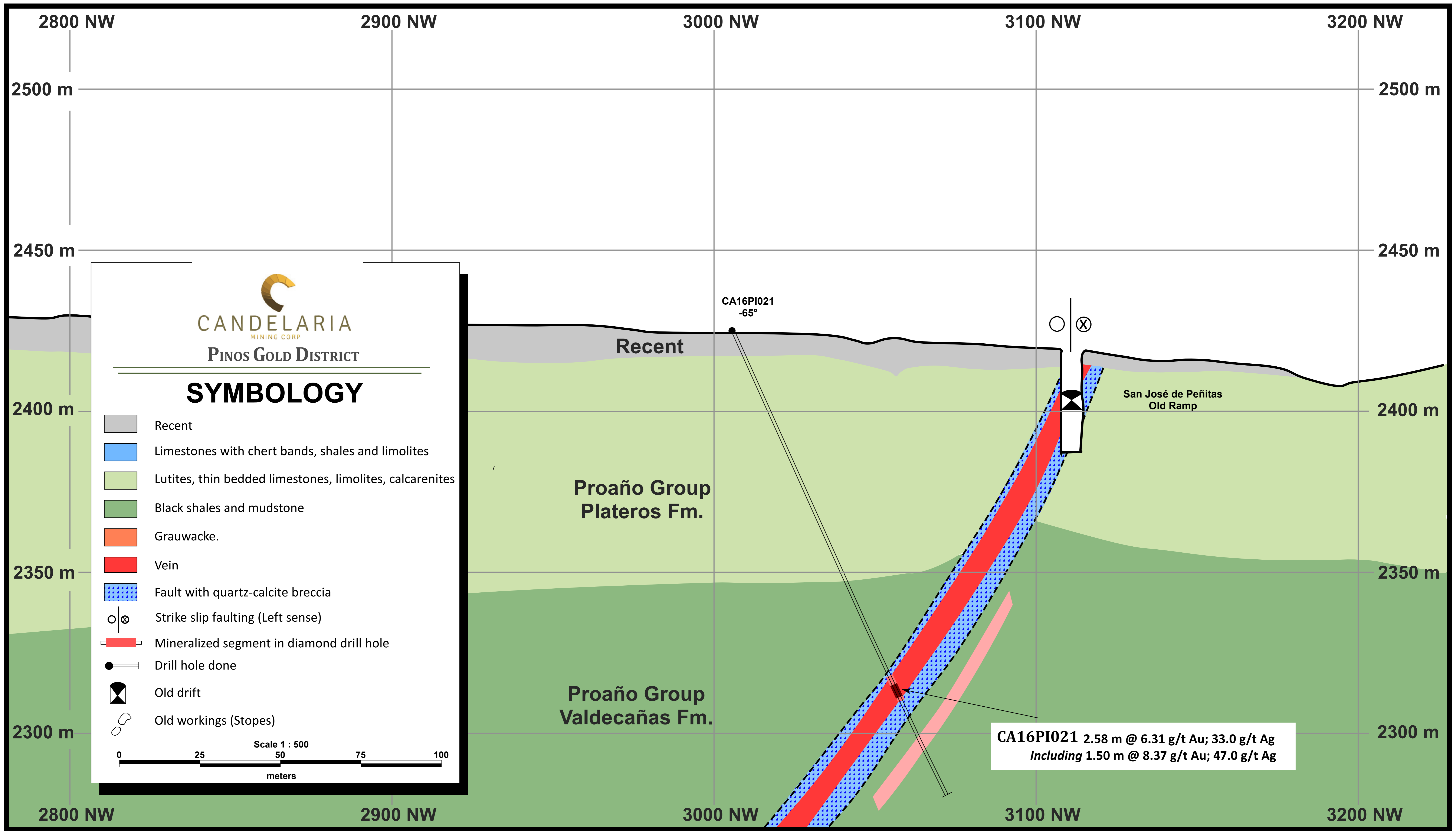
PINOS DISTRICT, TRANSVERSAL SECTION 8040 NE (LOOKING NW) SAN JOSÉ DE PEÑITAS CINCO ESTRELLAS VEINS SYSTEM
