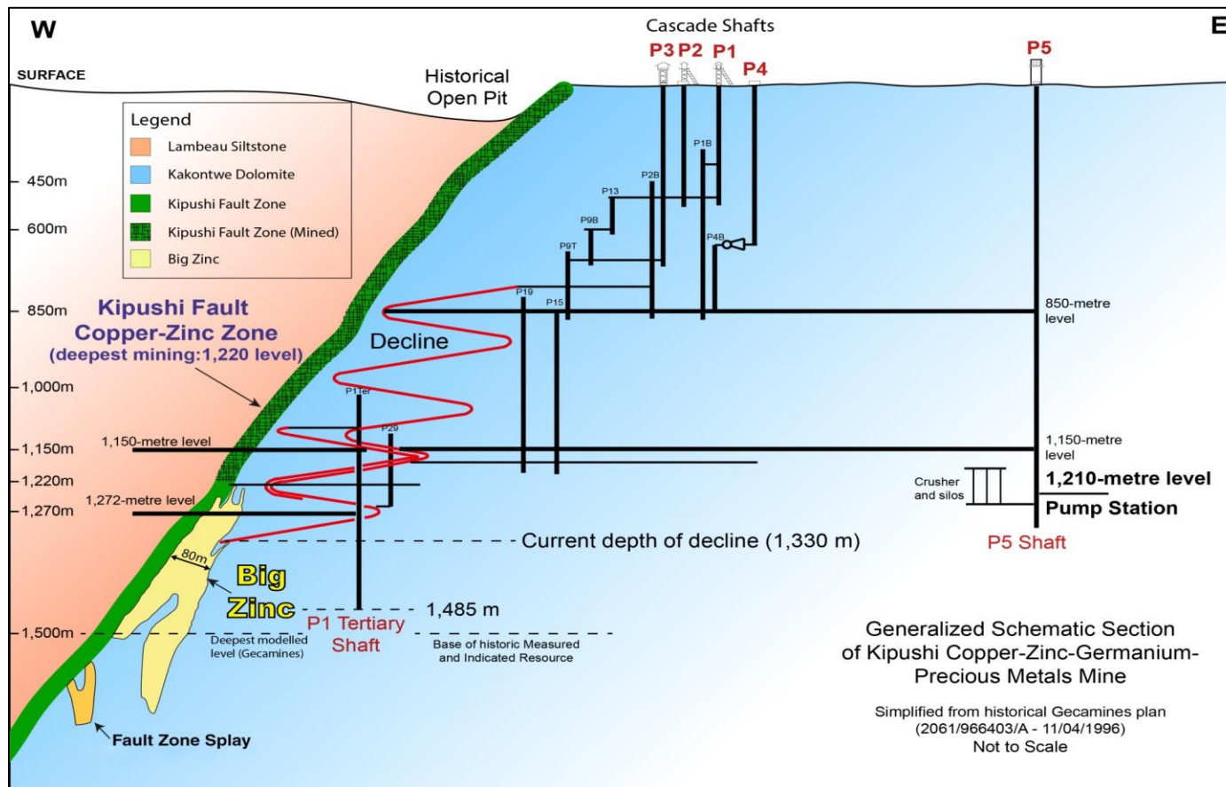
Figure 1. Schematic section of Kipushi Mine.
