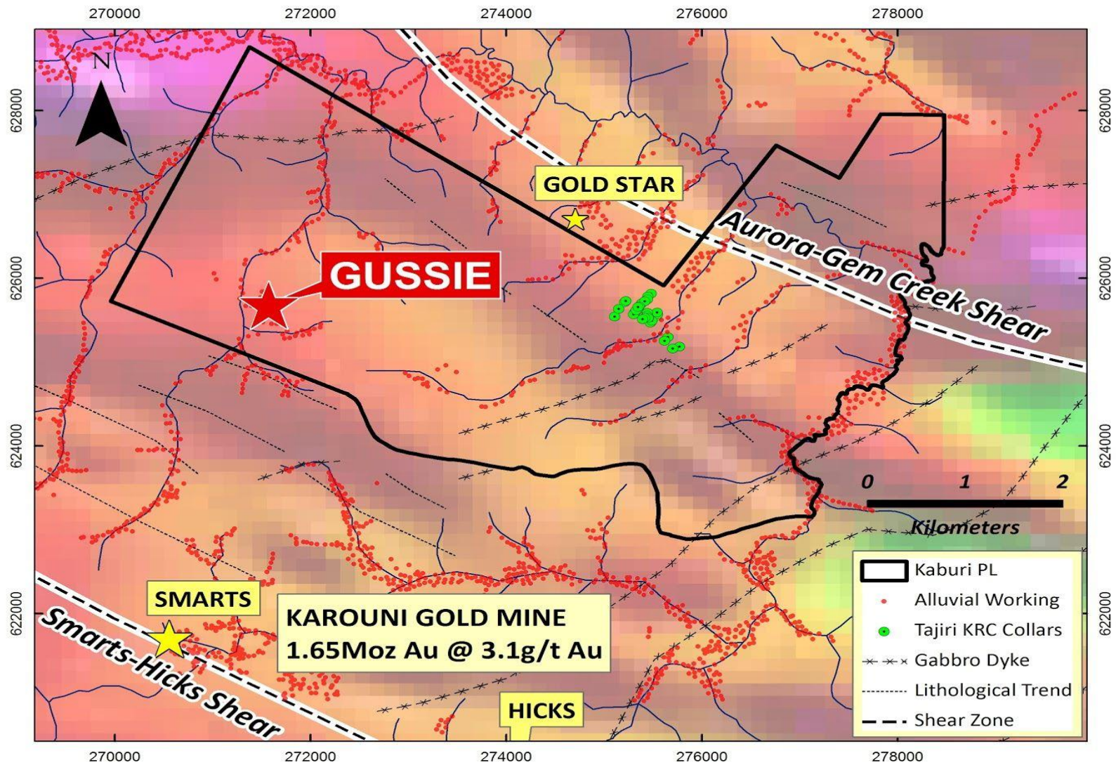
Figure: Gussie prospect drill target within the Kaburi Project boundary on regional airborne magnetics.
