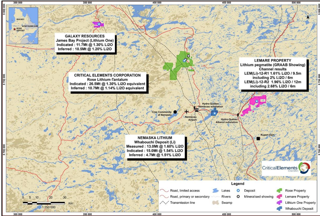
Figure 1. Location of the Lemare spodumene project in the James Bay region of Quebec, Canada, in relation to several advanced lithium projects. Nemaska Lithium's Whabouchi project is only 30 km west of Lemare.
