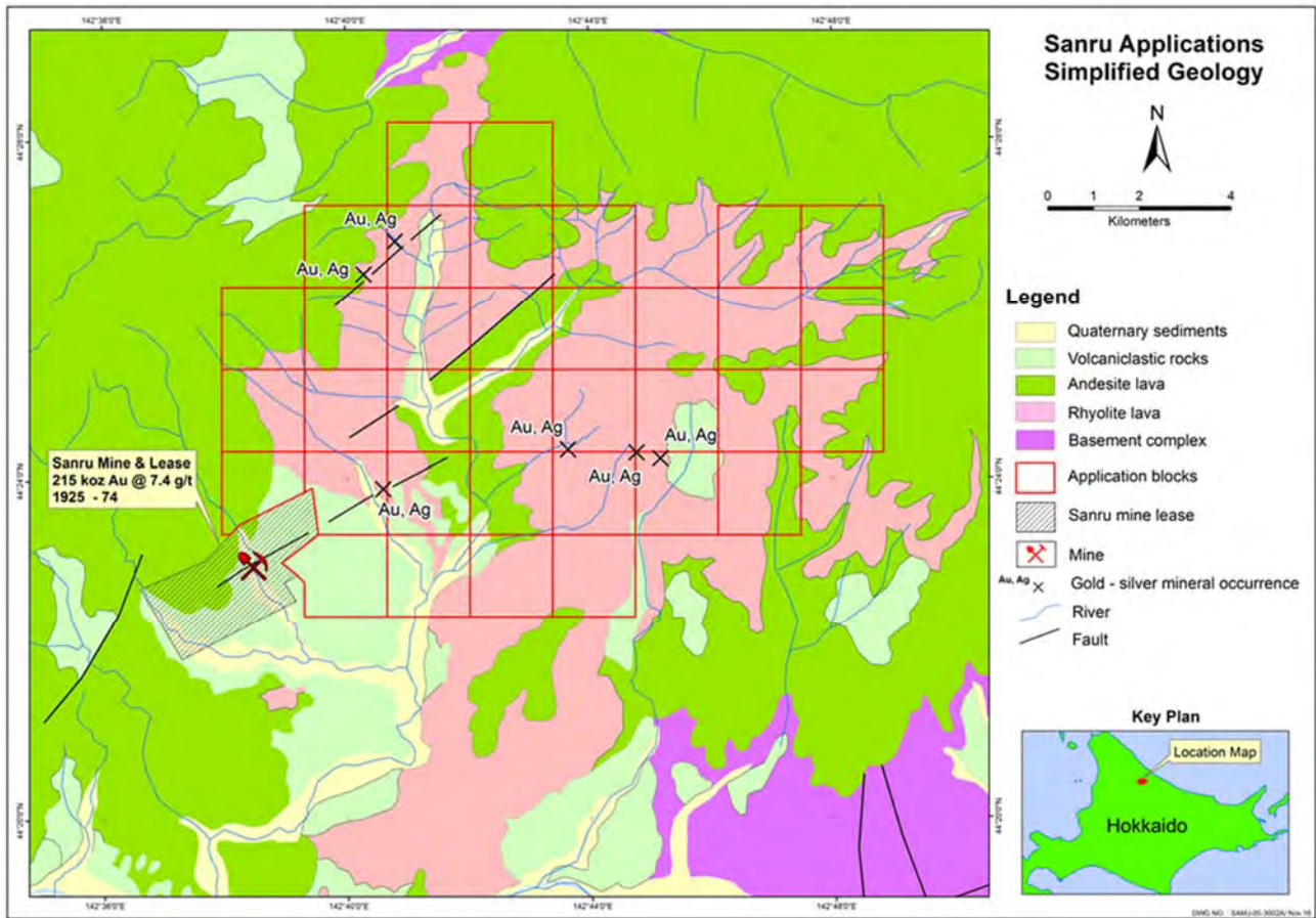
Figure 2, Japan Gold, Sanru Applications simplified geology.
