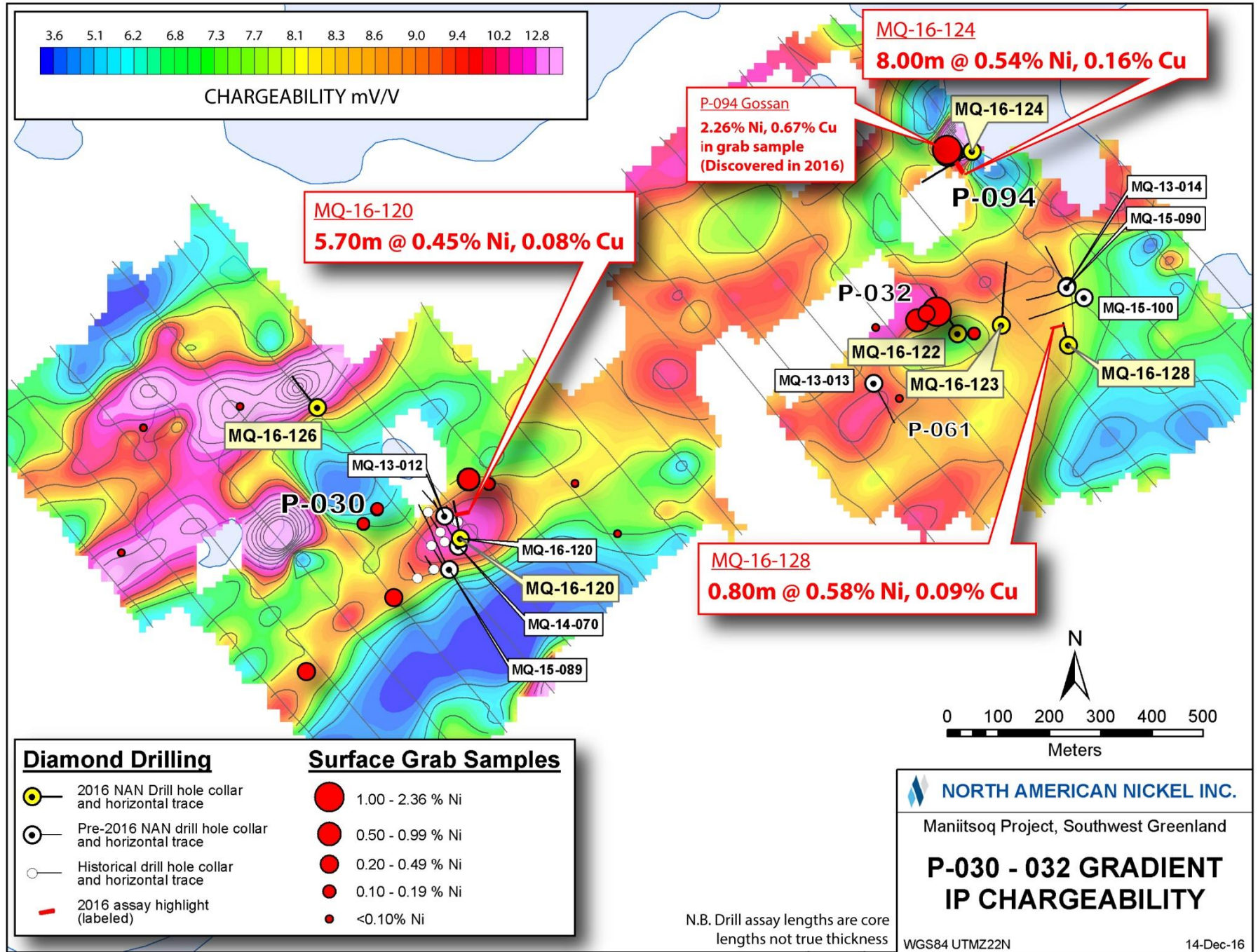
Figure 3: P-030 - P-032 target area gradient IP chargeability.
