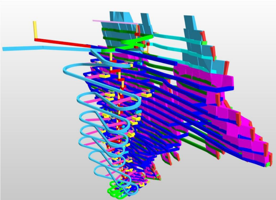
Figure 1: Mpama North Life of Mine Design and Layout
