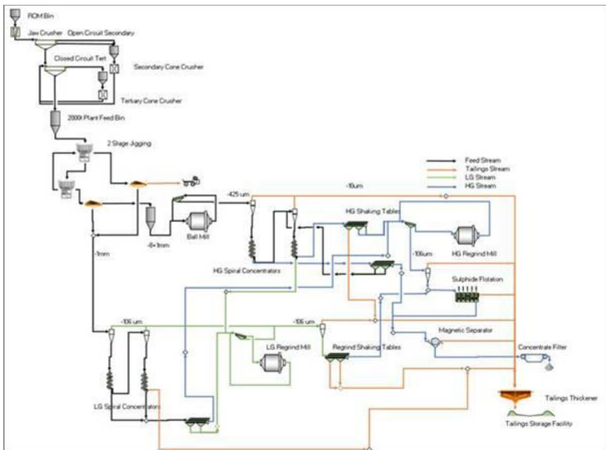
Figure 3: Bisie Process Flow Sheet
