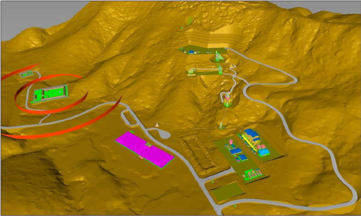
Figure 4: 3D View of Overall Block Plan
