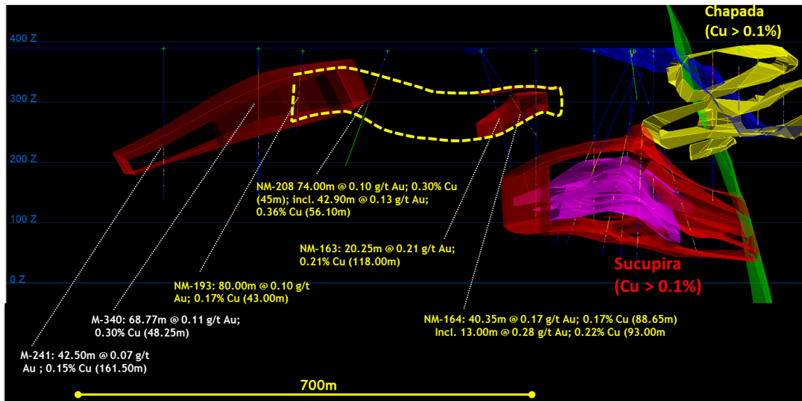
Figure 10: Northwest to southeast cross section showing the location of the Baru deposit (yellow dashed line) relative to the Sucupira deposit.
