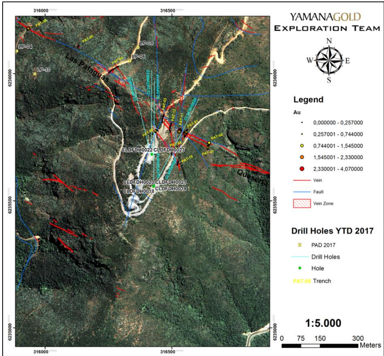
Figure 4: Plan view of the Las Pataguas target shows vein segments in red and drill hole traces in light blue, mapped vein surface exposures in red.
