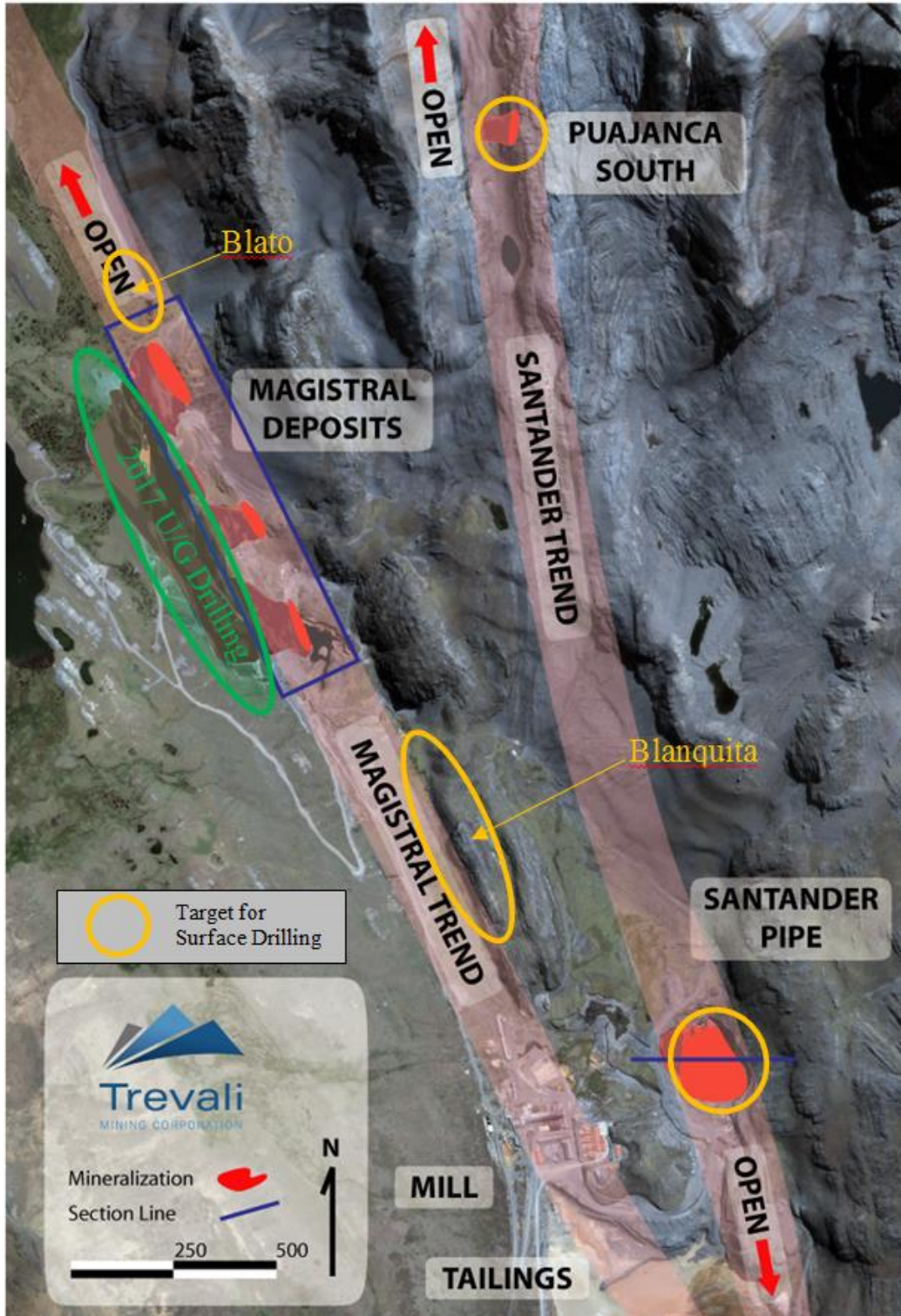
Figure 1: Location of 2016 Capped Measured, Indicated and Inferred Mineral Resources (red) at Santander Mine; and 2017 Drill Target areas (orange – surface drilling; green – underground drilling).
