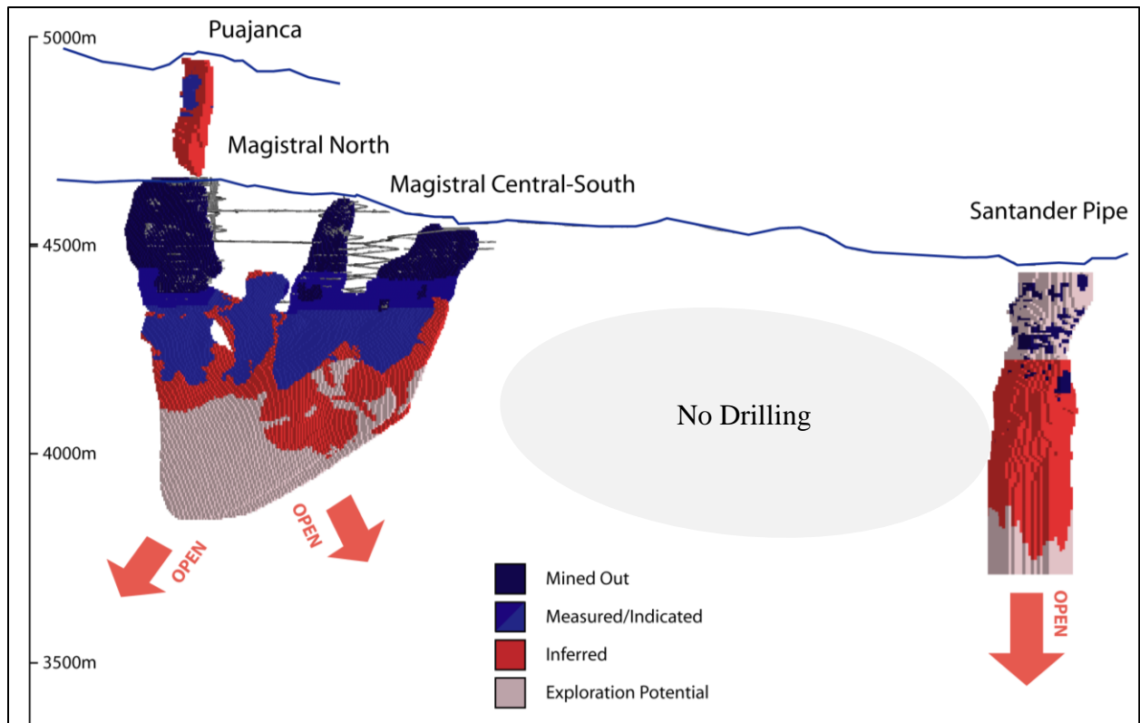
Figure 3: Longitudinal Section (Looking East) of Magistral Deposits, Puajanca and Santander Pipe with 2017 Mineral Resources – illustrating successful replacement of mined inventory during the period.
