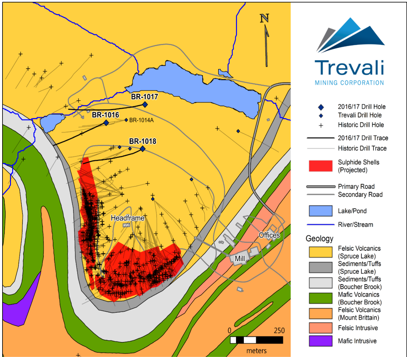
Figure 1: Geologic map with projected sulphide mineralization.
