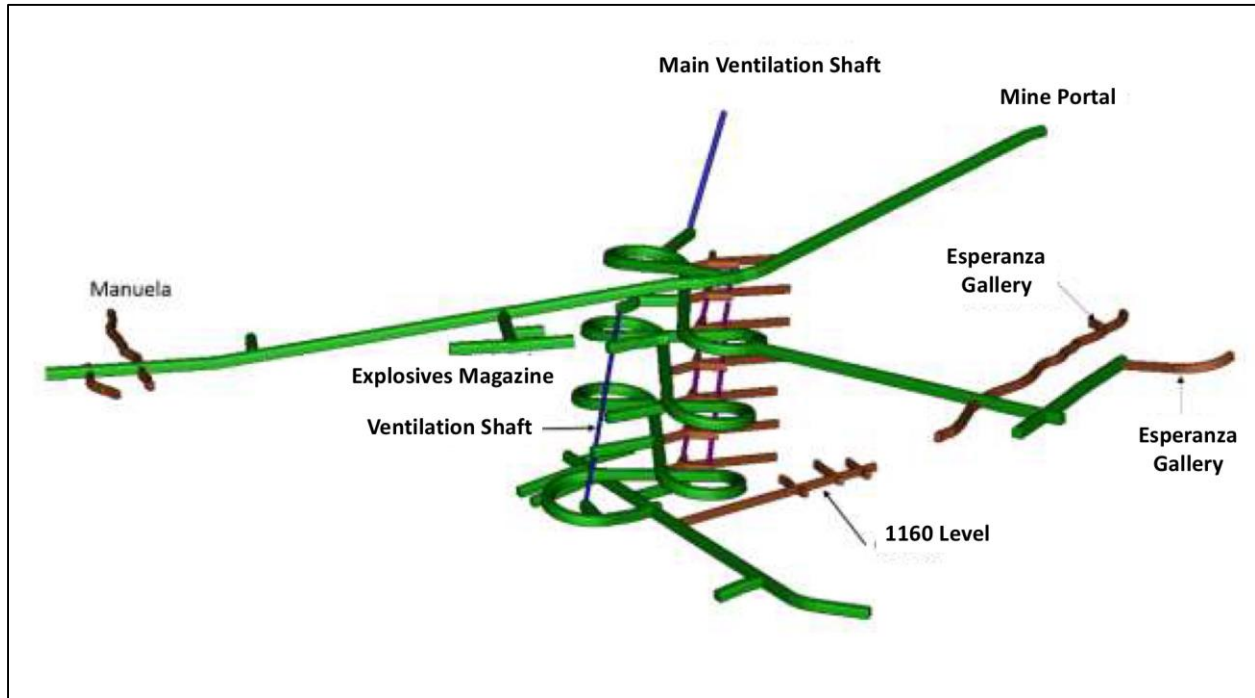
Figure 1 – Guaico Underground Tunnelling Advances to February 28, 2017
