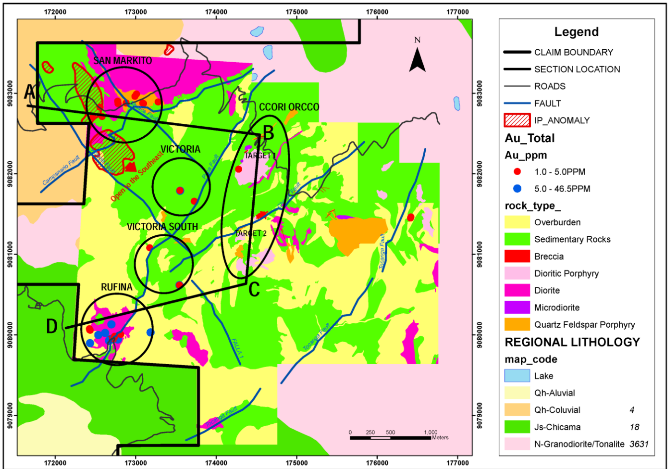
Figure 1 - Geological Plan Map of La Victoria Property showing Locations of Major Target Areas
