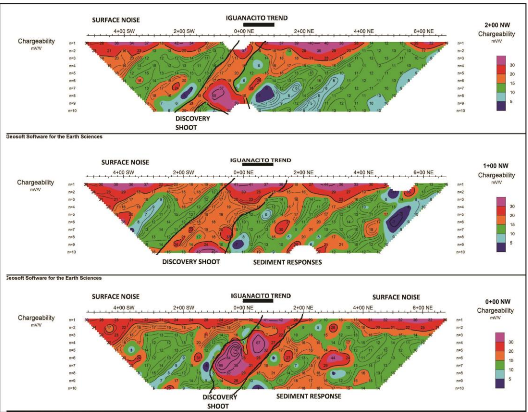
Figure 3: IP Chargeability Pseudo Sections - Central Shoot. Black lines highlight the chargeability responses of the Central Shoot
