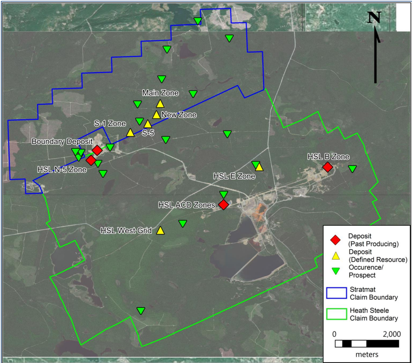
Figure 1: Location map of the Heath Steele and Stratmat claim groups showing location of historic mine production, defined resources and known prospects.
