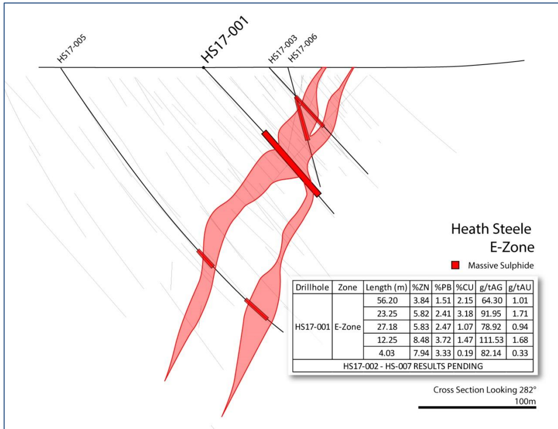
Figure 4: Cross section through the Heath Steele E-Zone, looking WNW.
