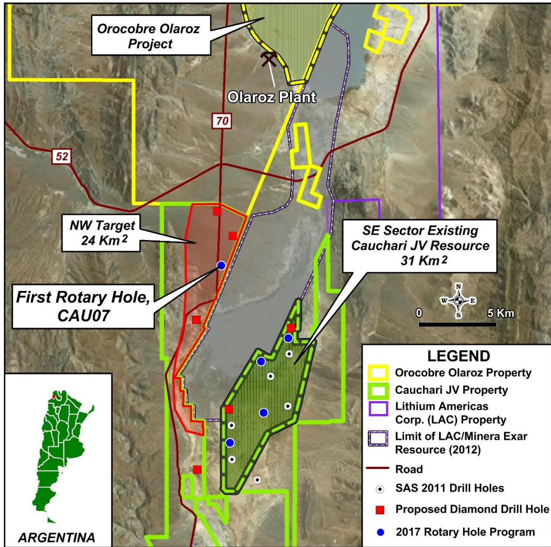
Figure 1: Location of the phase 1 drill holes relative to previous drilling
