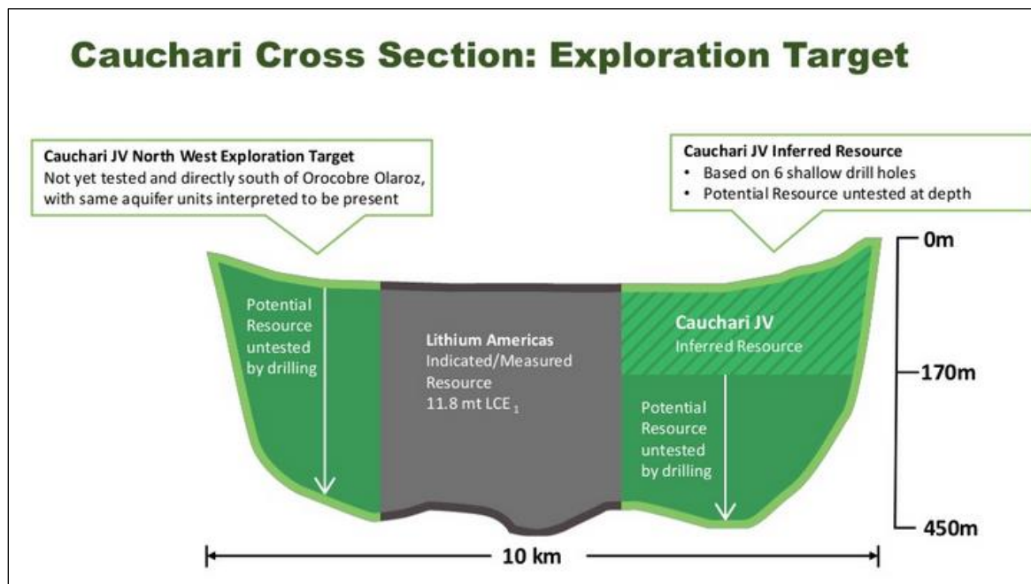
Figure 3: The location of the Cauchari drilling areas relative to the Lithium Americas Corp. lithium resource
