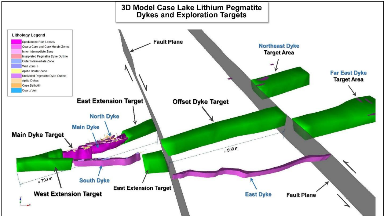
Figure 2 3D model of Case Lake pegmatite exploration targets, looking north.
