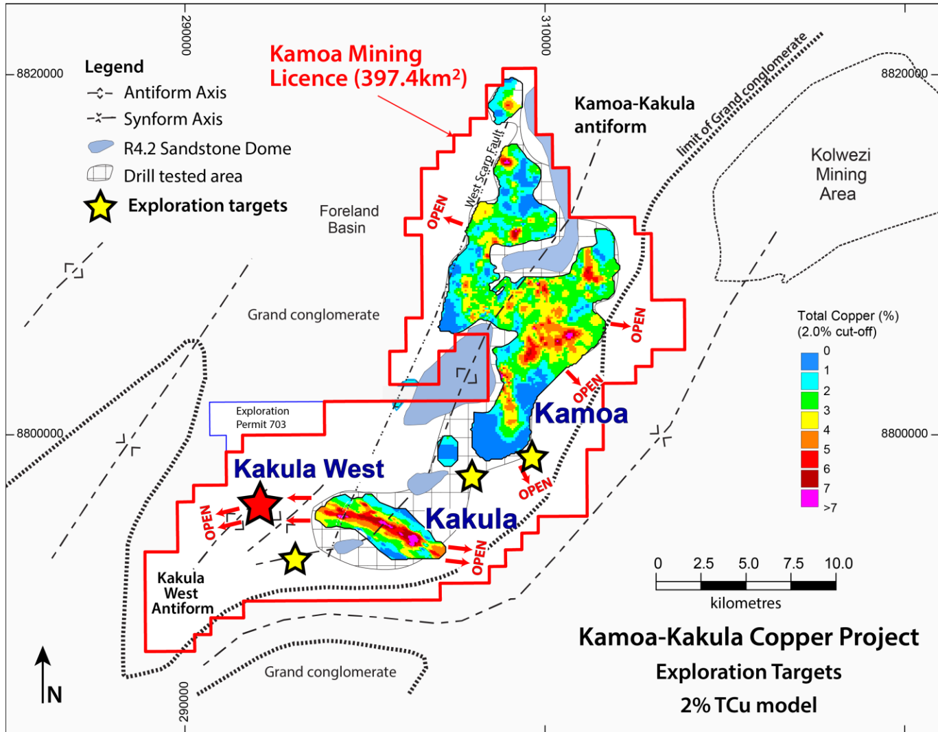
Figure 2. Kamoa-Kakula mining licence shows the copper grades of the Kamoa and Kakula Indicated and Inferred Mineral Resource areas, and the Kakula West Discovery.
