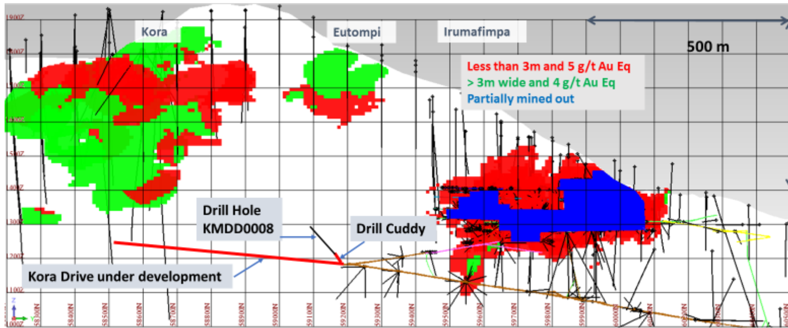
Figure 1 Long Section through the Irumafimpa and Kora Orebodies
