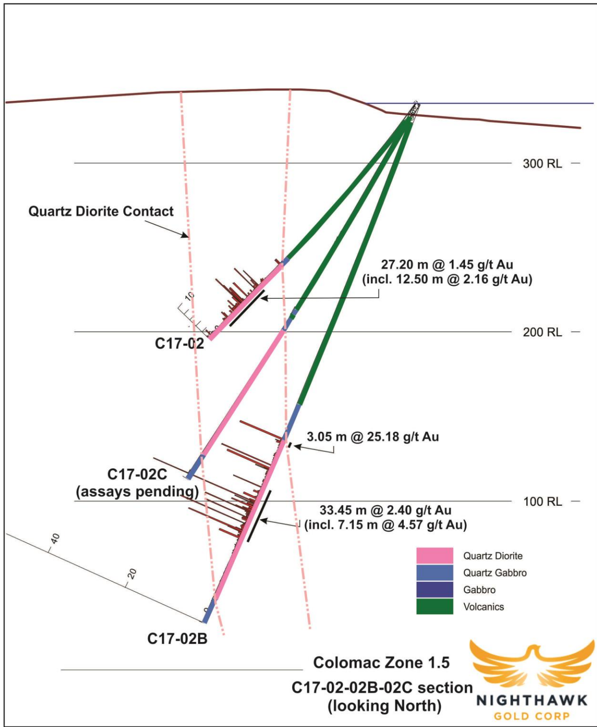
Figure 3. Cross Section – Drillholes C17-02, C17-02B, C17-02C
