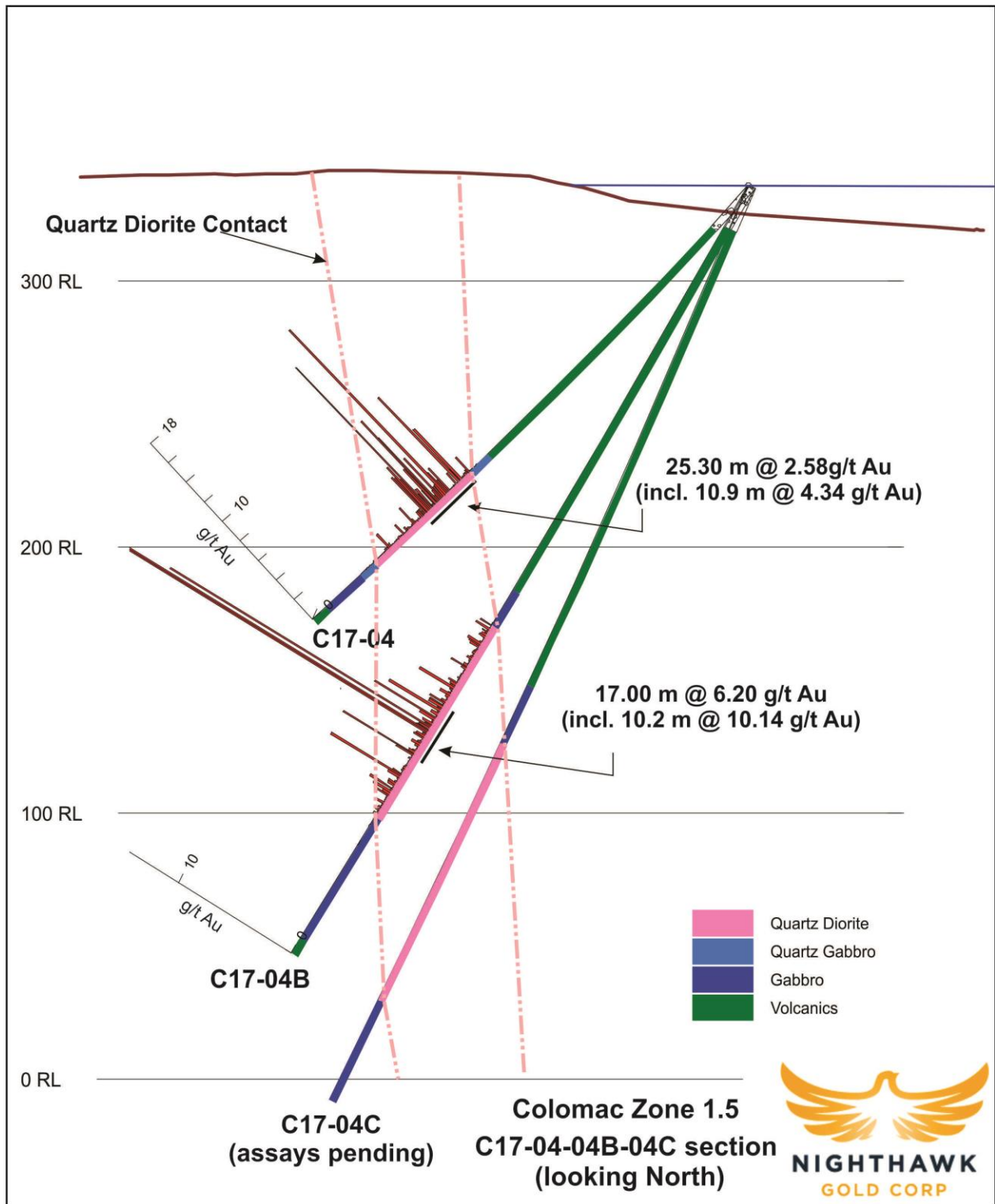
Figure 2. Cross Section - Drillholes C17-04, C17-04B, C17-04C
