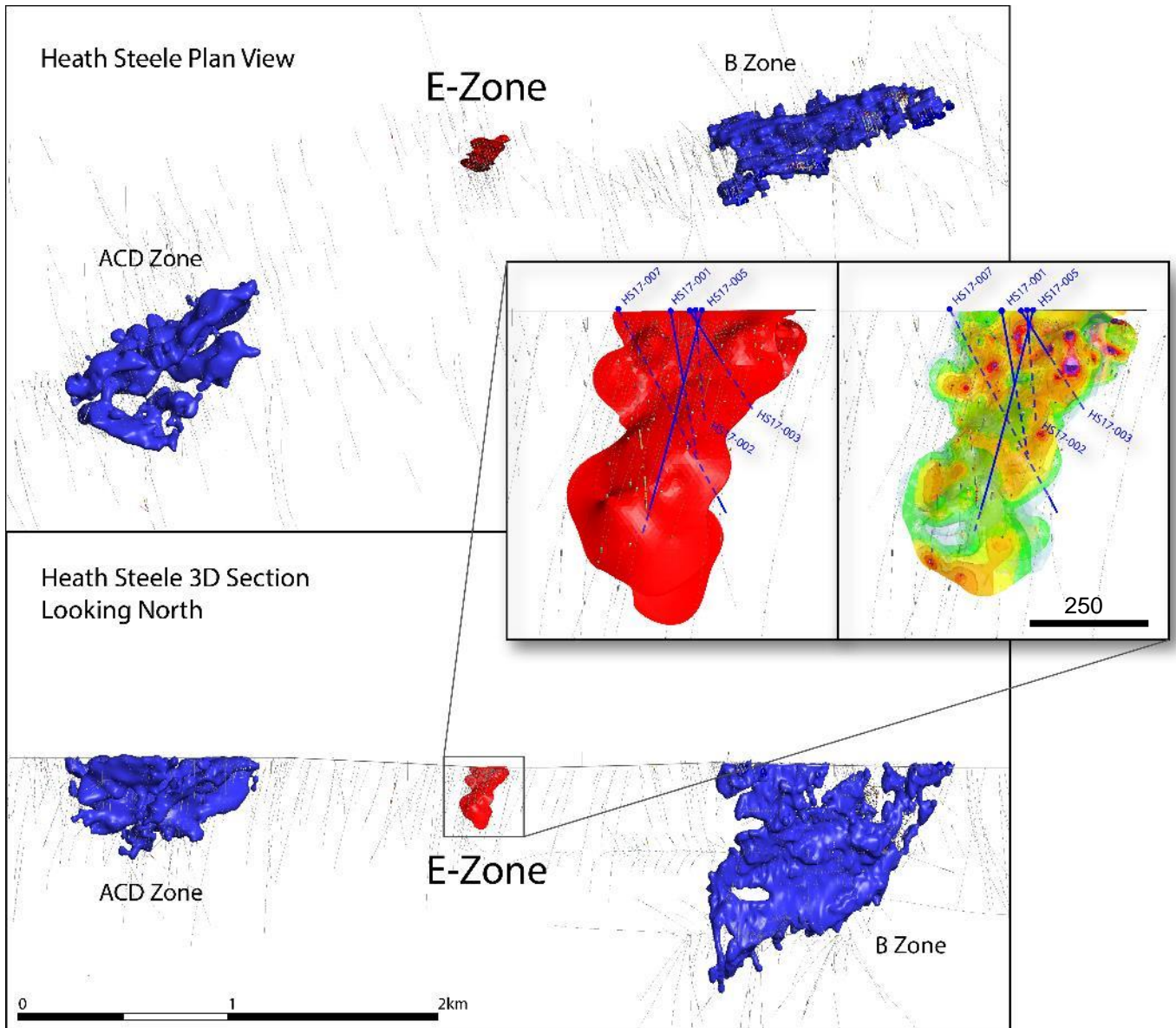
Figure 3: Various plan and 3-D section views of the Heath Steele drill hole data and the E-Zone.
