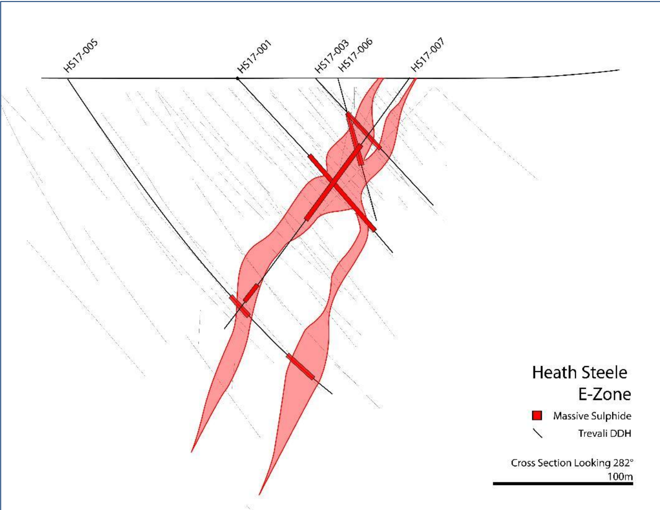
Figure 4: Cross section through the Heath Steele E-Zone, looking WNW, section width is 80 metres
