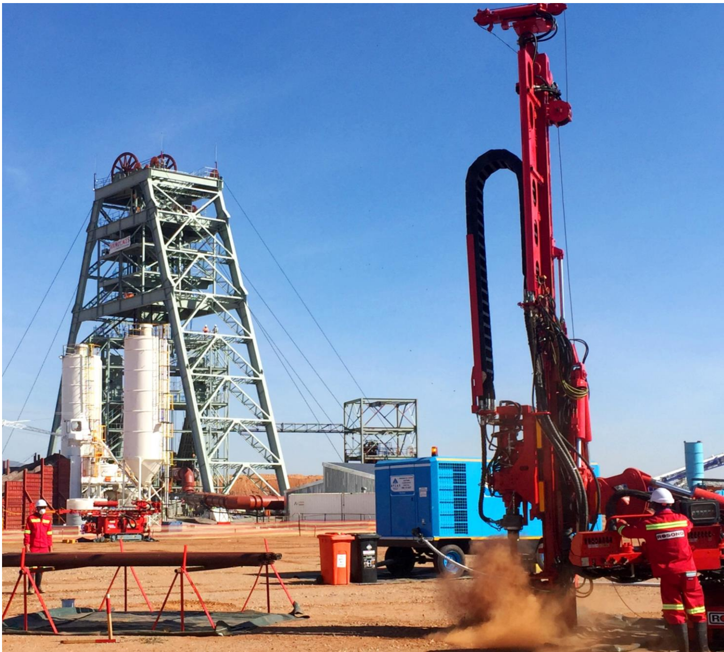
Photo 5: Shaft 2 early works underway.
