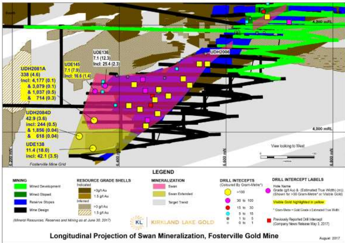
Figure 2. Longitudinal View – Swan Mineralization at Fosterville Gold Mine
