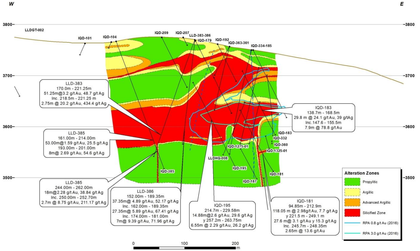
Figure 4: Alteration Section 700
