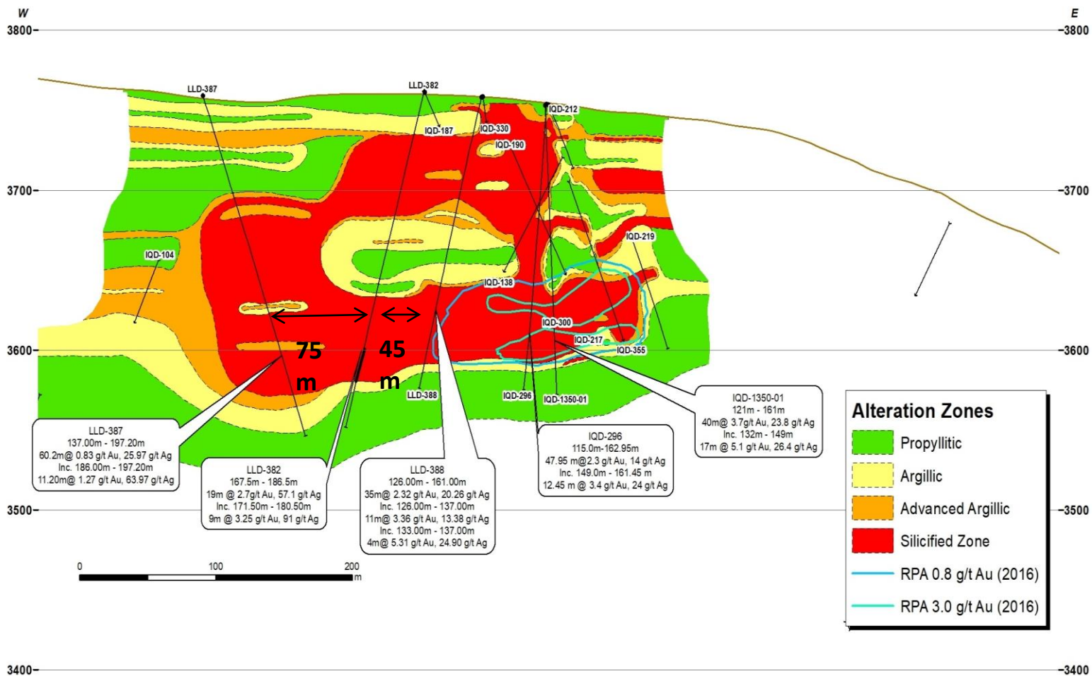
Figure 5: Alteration Section 800
