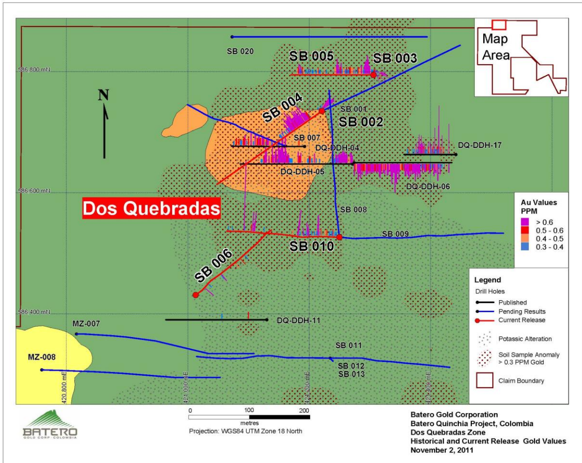
Figure 2 - Plan Map for Dos Quebradas drill hole locations
