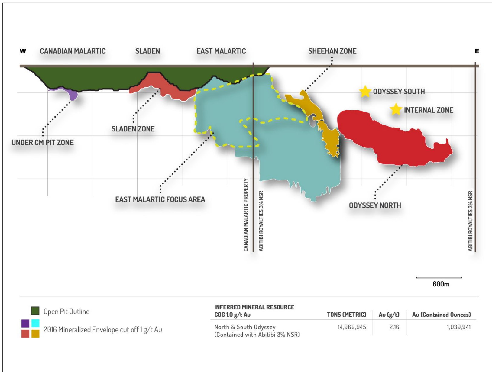
Fig. 3 – Schematic Longitudinal Section of the Canadian Malartic Mine & Abitibi Royalties 3% NSR
