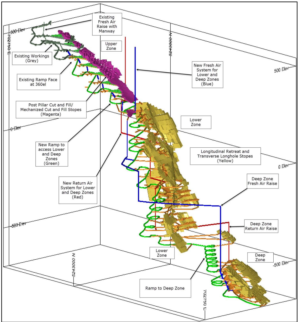
Figure 1: Halfmile 3D Mine Model Isometric View Looking Southwest
