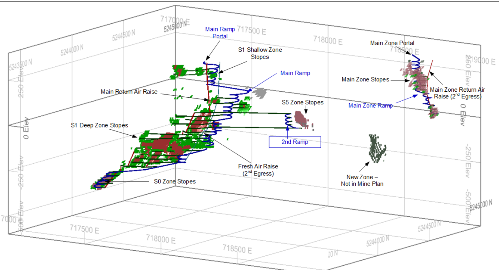
Figure 2: Stratmat 3D Mine Model Isometric View Looking Northeast
