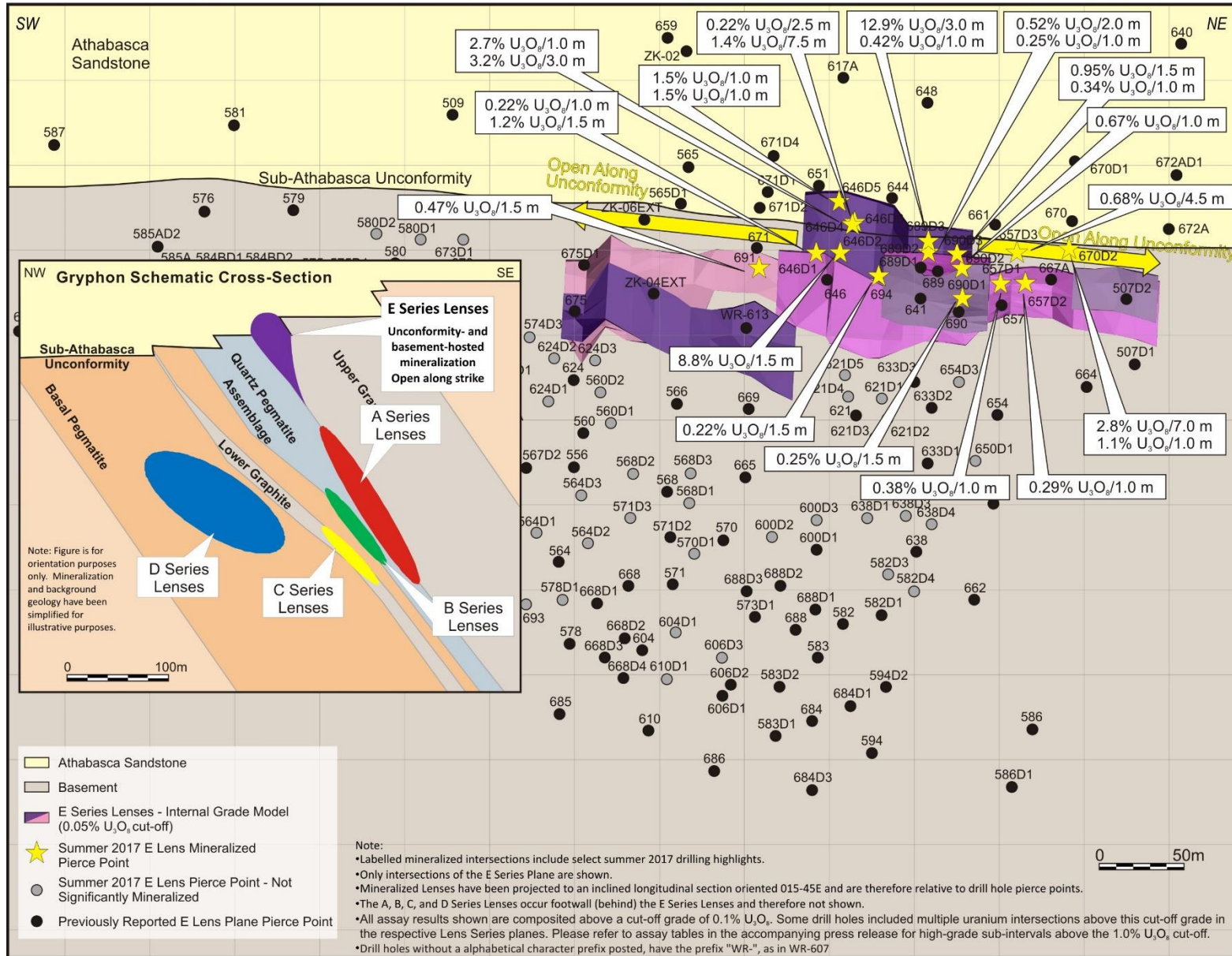
Figure 6: Inclined longitudinal section of the Gryphon E series lenses.
