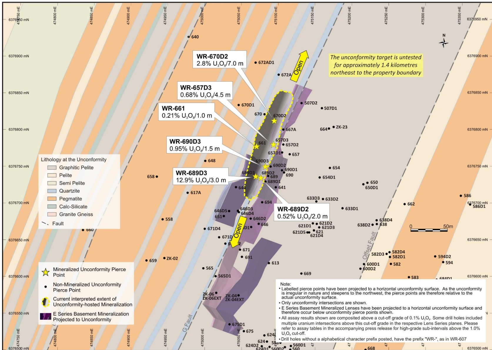
Figure 7: Plan map of the Gryphon E series lenses (unconformity and upper basement mineralization).
