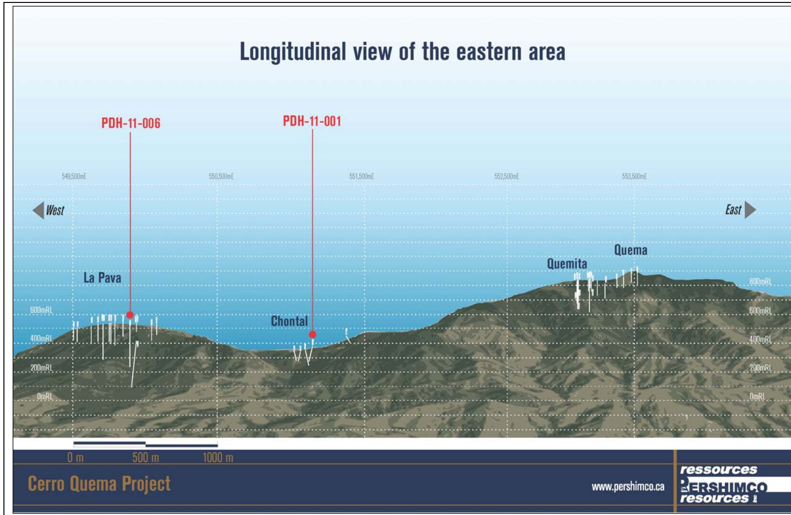
Figure 1 : Longitudinal View of the 4-kilometre long La Pava, Chontal and Quema-Quemita segment of the 17-kilometre Cerro Quema Gold-Copper Trend. Drill holes PDH-11-006 at La Pava and PDH-11-001 at Chontal are highlighted in red.
