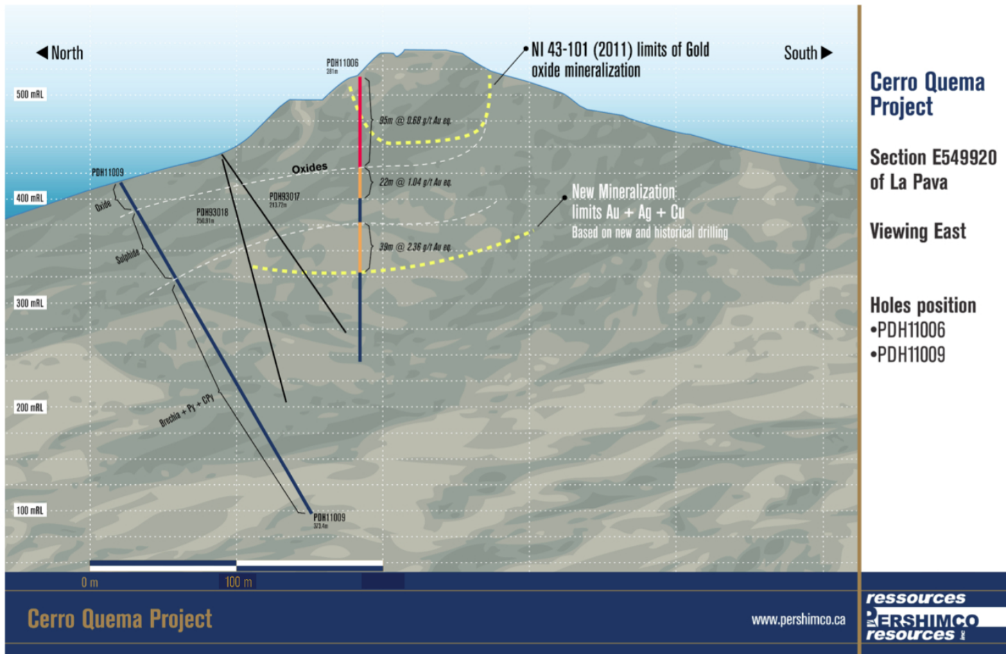
Figure 2 : La Pava Section 549920E, looking east showing the position of drill holes PDH-11-006 and PDH-11-009. The section also outlines the depth limit of the gold oxide mineralization as outlined in the 2011 NI 43-101 Technical Report by Scott Wilson, and the limits of the oxide and sulphide mineralization based on the current drilling.
